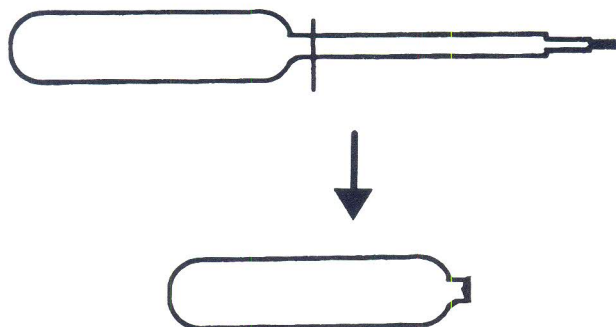
Fig. 3. Cutting off the bulb from a one-piece plastic pipette.
